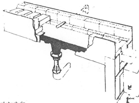
FIGURE 1—Thermal shock rig.
